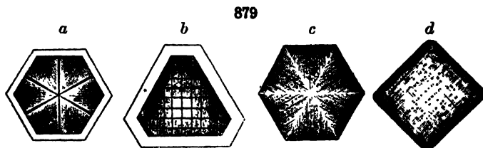
Sections of crystals of haüynite (after Mühl)
